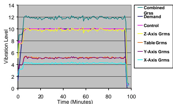
Fig. 7. Random vibration profile
