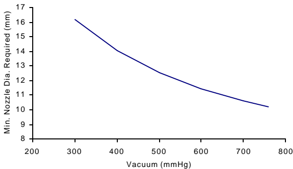
Fig. 10. Nozzle diameter vs. vacuum
