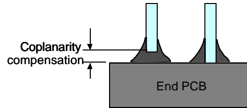
Fig. 4. Compensation for coplanarity
