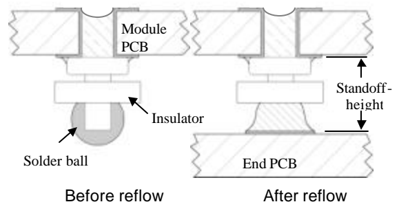
Fig. 2. Sketches of a CPSB connector before and after end assembly reflow.
