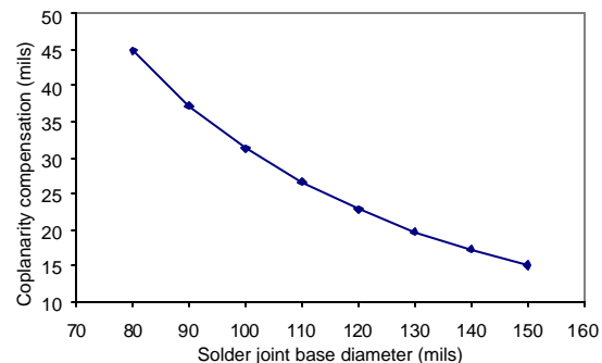
Fig. 5. Compensation for coplanarity
