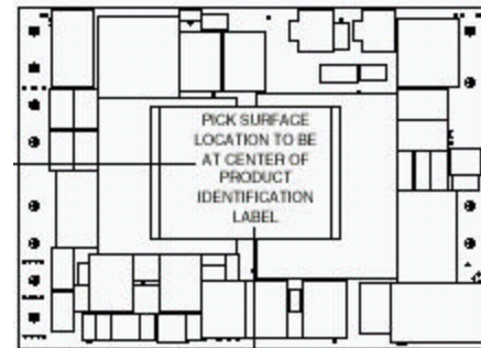
Fig. 8. Example of designated pick-and place device in TEPS power modules.
