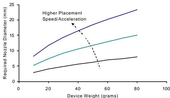
Fig. 11. Nozzle diameter vs. speed/acceleration
