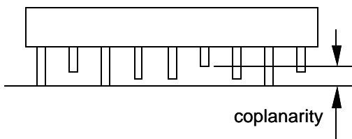
Fig. 3. Definition of coplanarity
