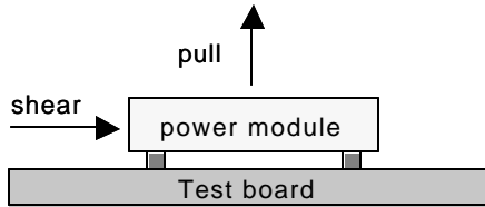
Fig. 6. Sketch of pull and shear test setup
