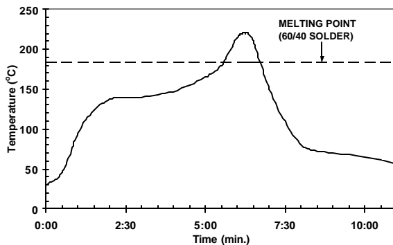
Fig. 12. Sample reflow profile
