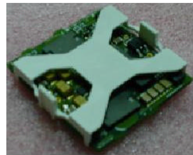
Fig. 9. Example of pick-and place fixture in TEPS power modules
